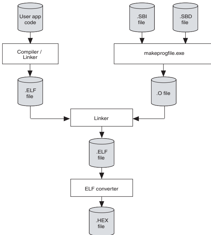
Figure 1. Using Run-from-Flash Mode with the Excalibur Bootloader
