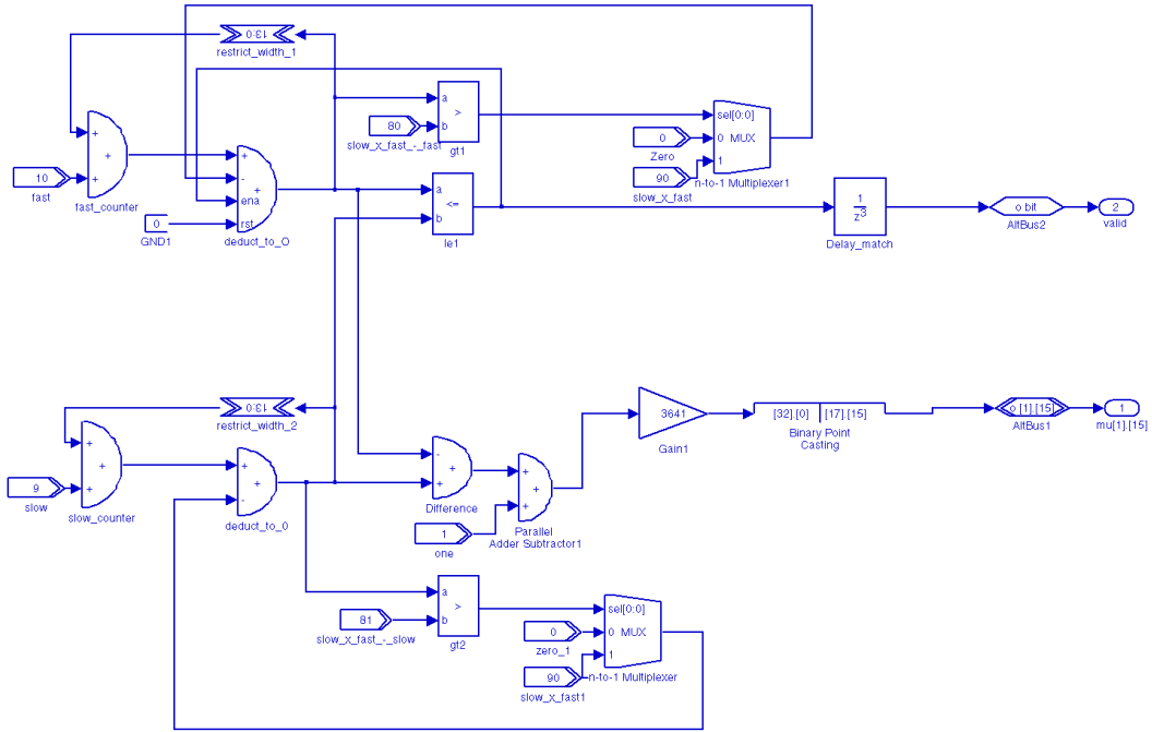
Figure 2. μ Generator Schematic
