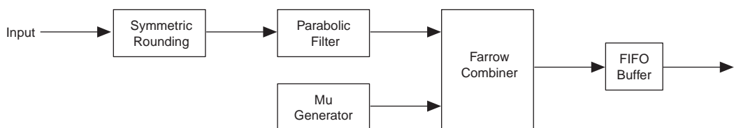
Figure 1. Block Diagram
