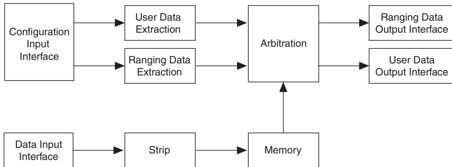
Figure 2. Block Diagram
