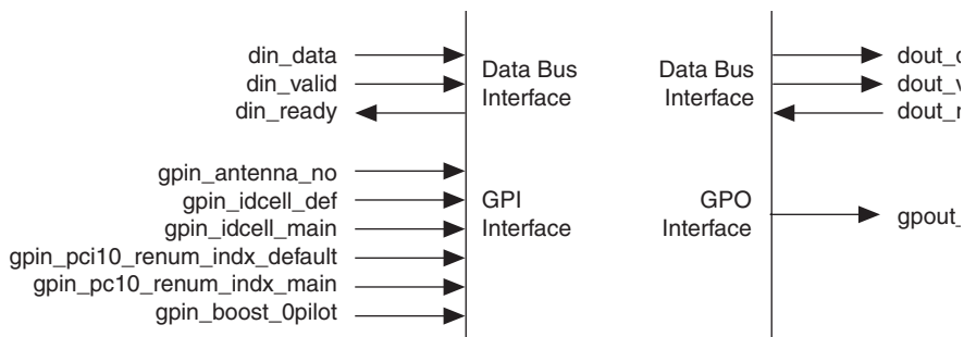
Figure 4. Subchannelization Design Interfaces
