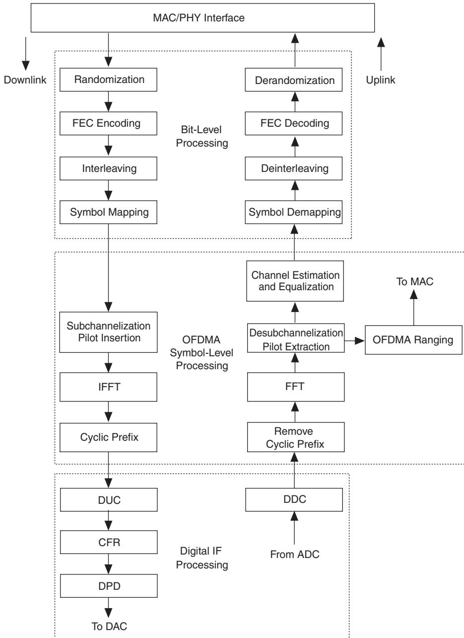
Figure 1. WiMAX PHY Implementation
