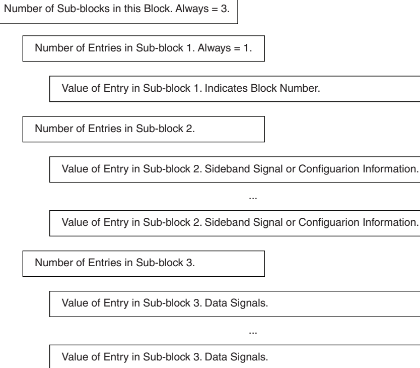
Figure 7. Structure of Single Block in File
