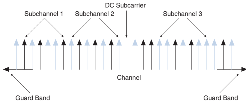
Figure 2. OFDMA Frequency Description
