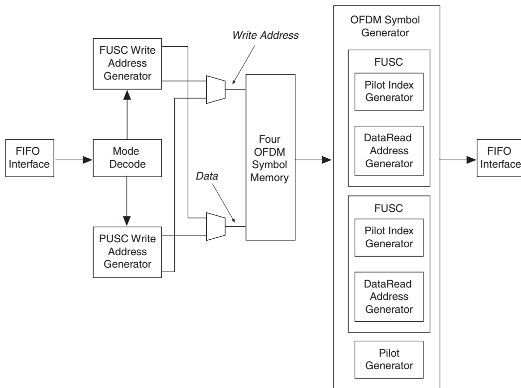
Figure 3. Subchannelization Block Diagram
