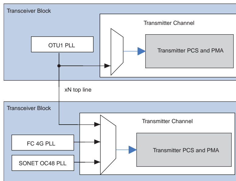
Figure 3. Example Design Placement Scheme
