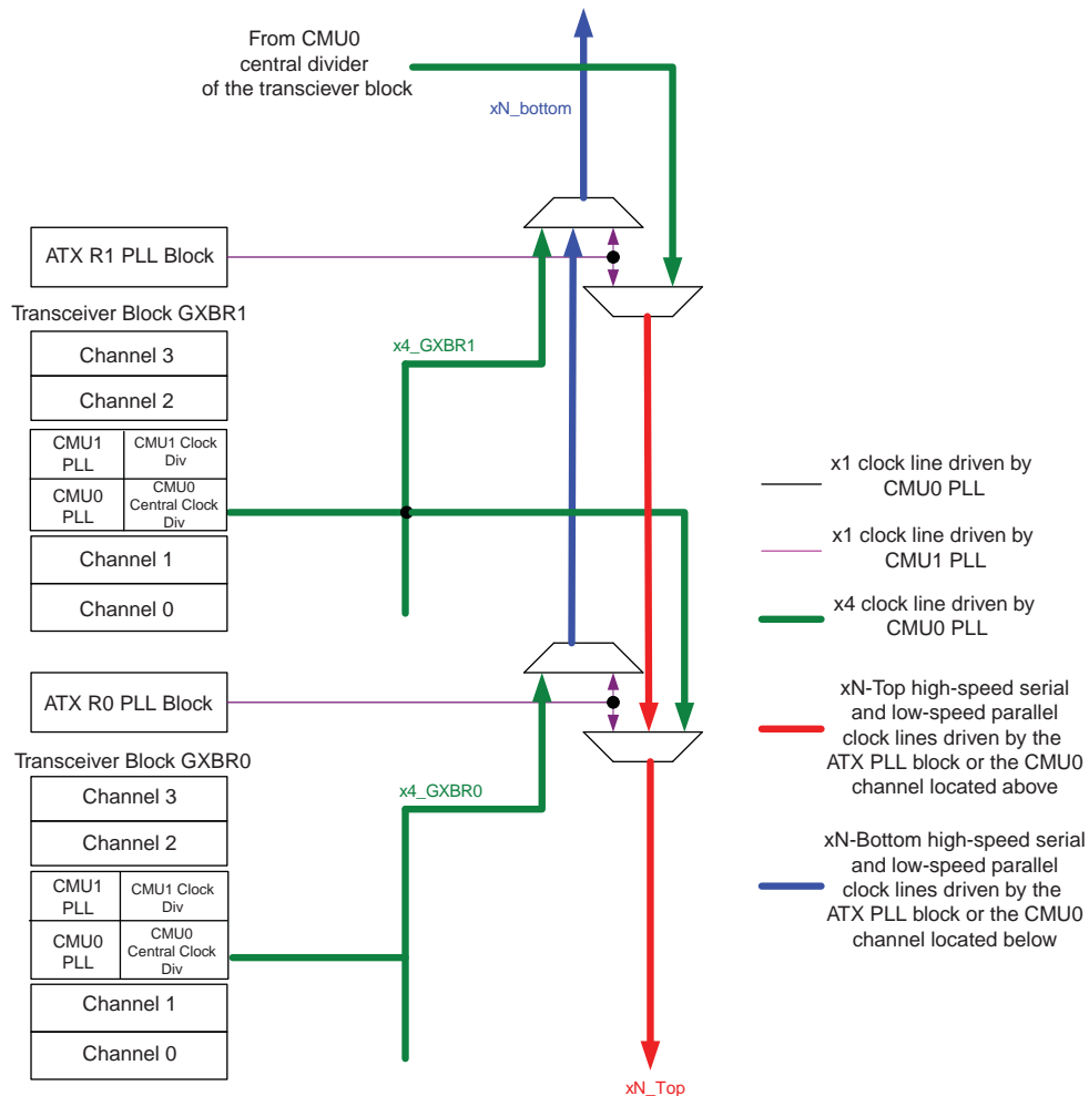
Figure 1. \times N Line Connections
