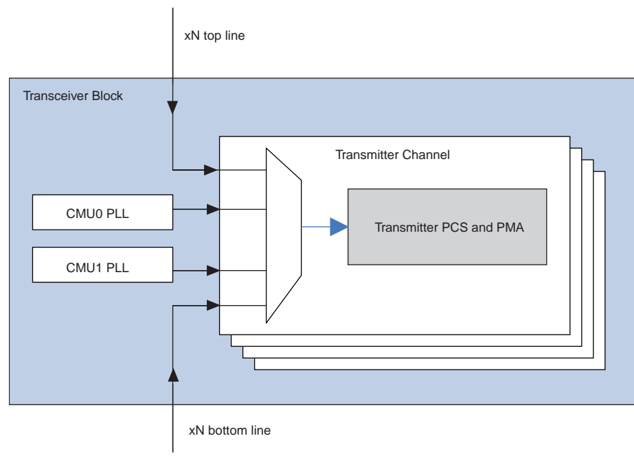
Figure 2. Number of PLLs Connected to a Transmitter Channel
