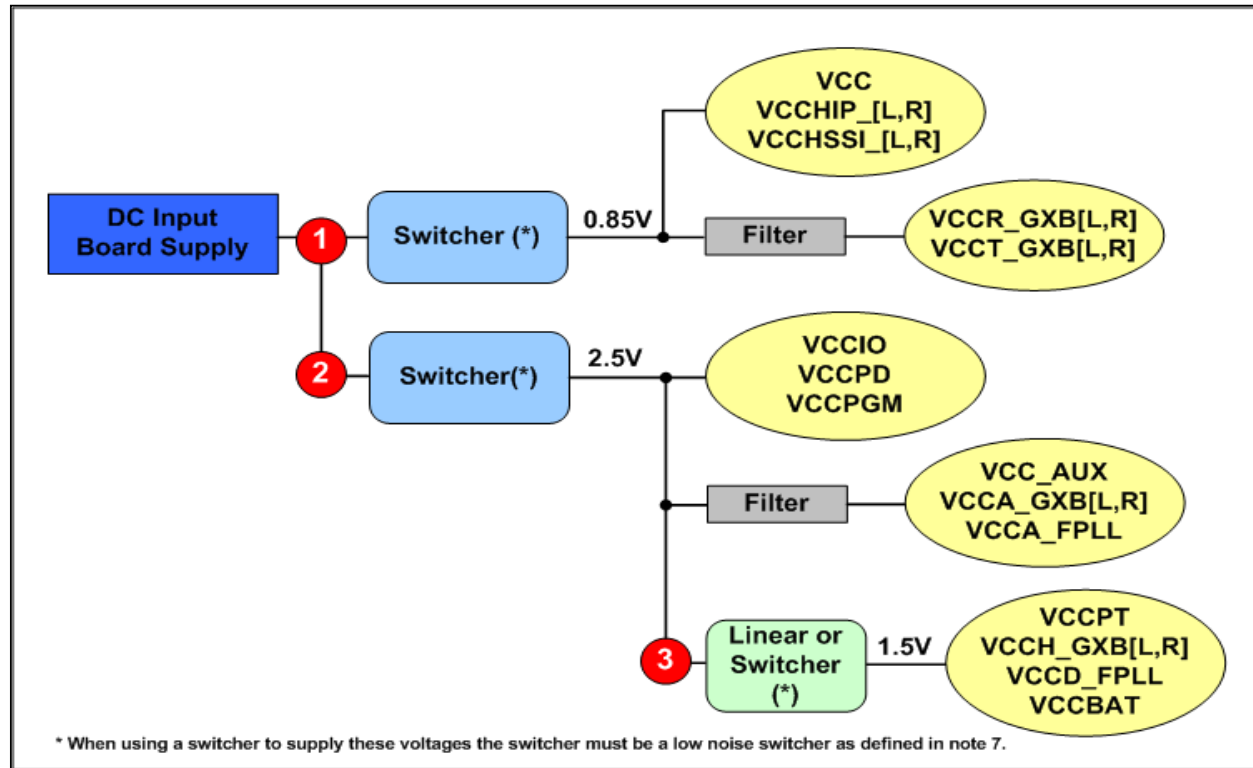
Figure 1. Example Power Supply Block Diagram for Stratix V Transceivers with Data Rates <= 6.5Gbps
