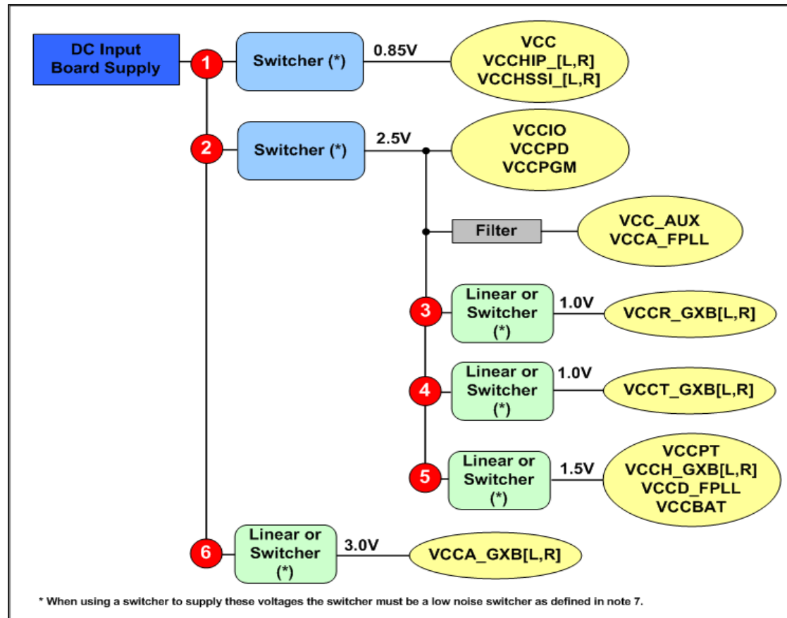
Figure 3. Example Power Supply Block Diagram for Stratix V Transceivers with Data Rates Greater than 12.5 Gbps
