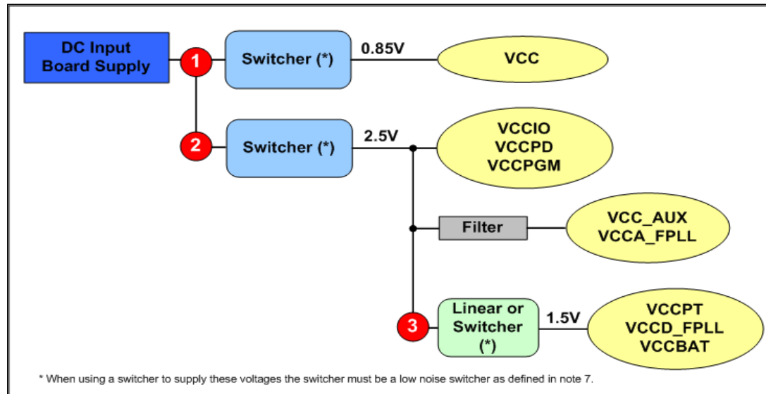
Figure 4. Example Stratix V E Power Supplies Block Diagram
