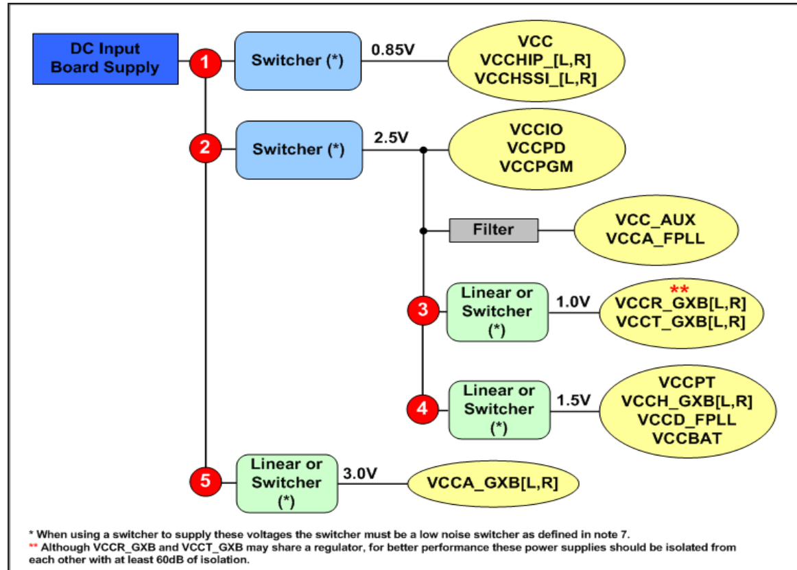
Figure 2. Example-Power Supply Block Diagram for Stratix V Transceivers with Data Rates Between 6.5 Gbps and 12.5Gbps
