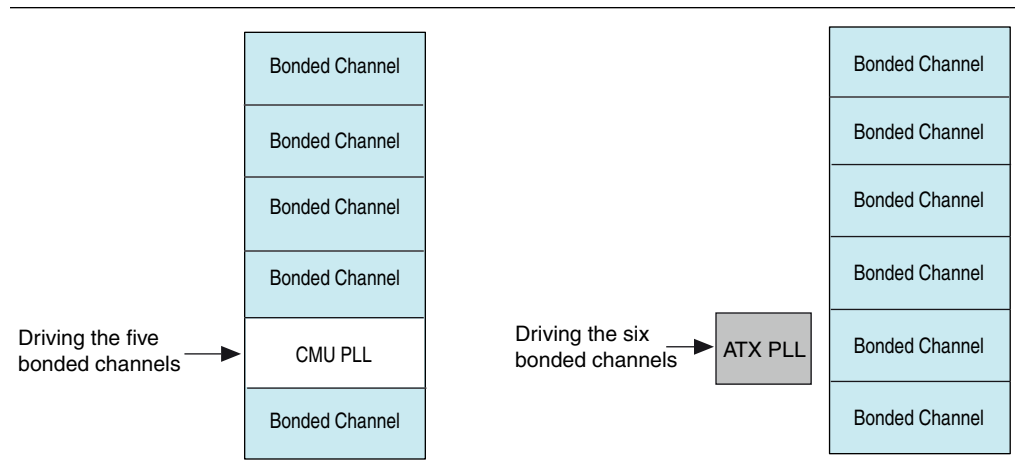
Figure 12. Bonded Channels Using a CMU PLL or a ATX PLL—Supported Configurations
