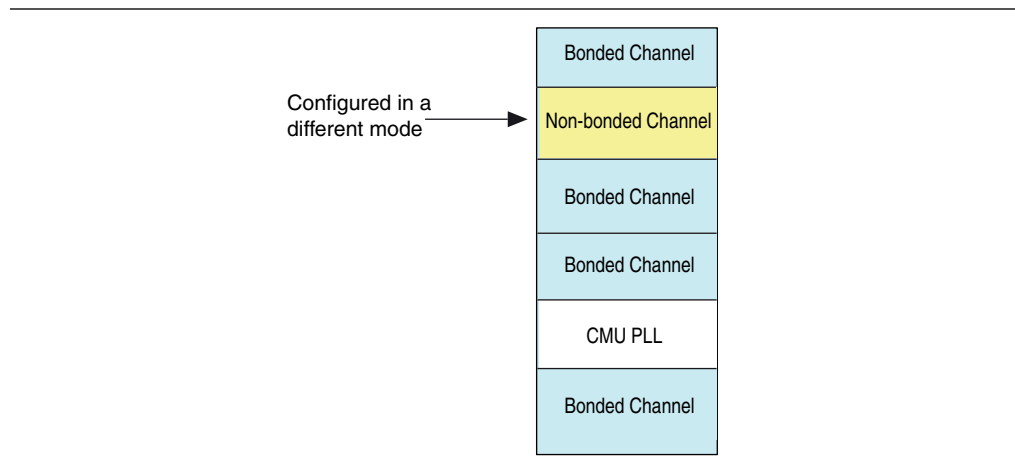
Figure 13. Bonded Channels—Non-Supported Configuration
