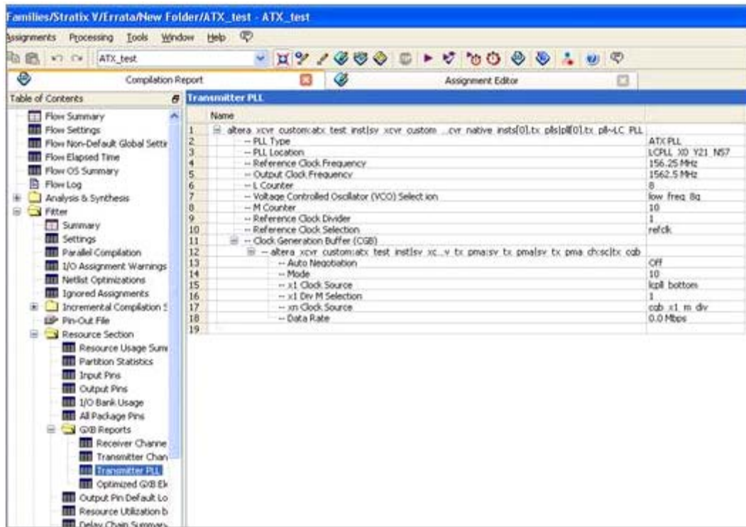
Figure 1. Fitter Report, Transmitter PLL Page
