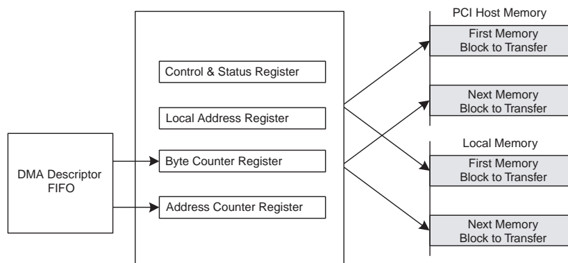
Figure 5. Chaining DMA Setup Sequence
