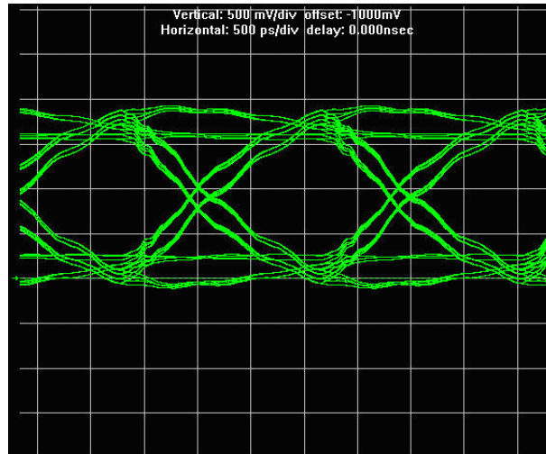
Figure 4-53. HyperLynx Simulation with a 16-mA Drive Strength Setting on the FPGA
