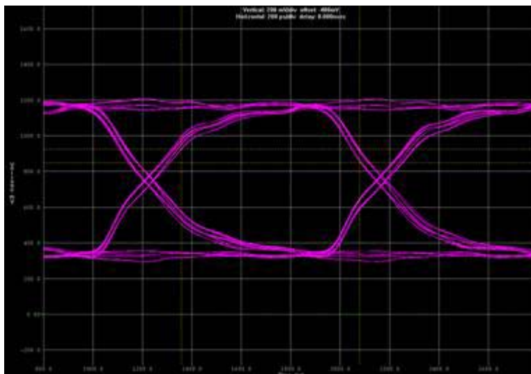
Figure 4-36. Simulated Write-Eye Diagram of a DDR3 SDRAM DIMM Using a 60-Ω ODT Setting
