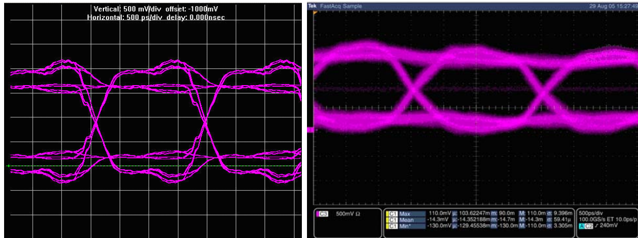
Figure 4-50. HyperLynx Simulation and Measurement of the Signal, FPGA Writing to Memory
