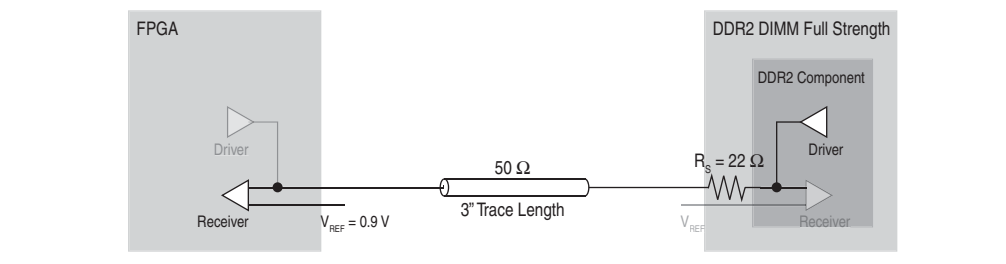
Figure 4-31. No-Parallel Termination Scheme, FPGA Reading from Memory
