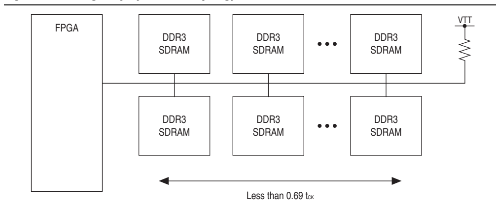
Figure 4-56. Single Fly-By Network Topology
