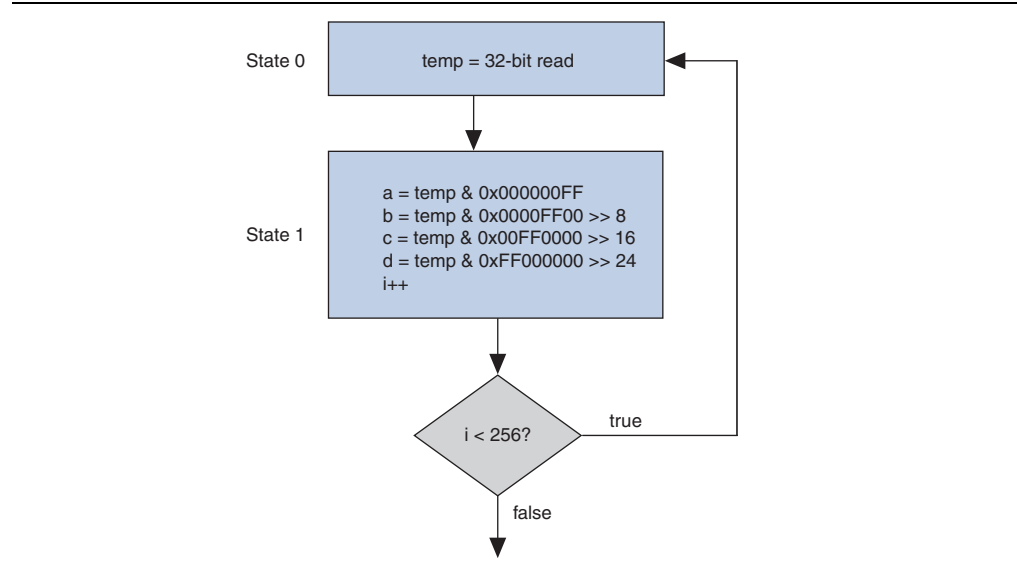
Figure 5-5. Wide Memory Access
