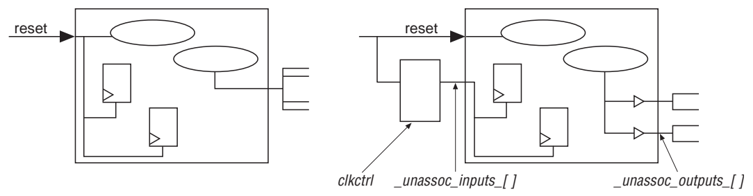
Figure 17-4. Creation of _unassoc_inputs_[] and _unassoc_outputs_[]
