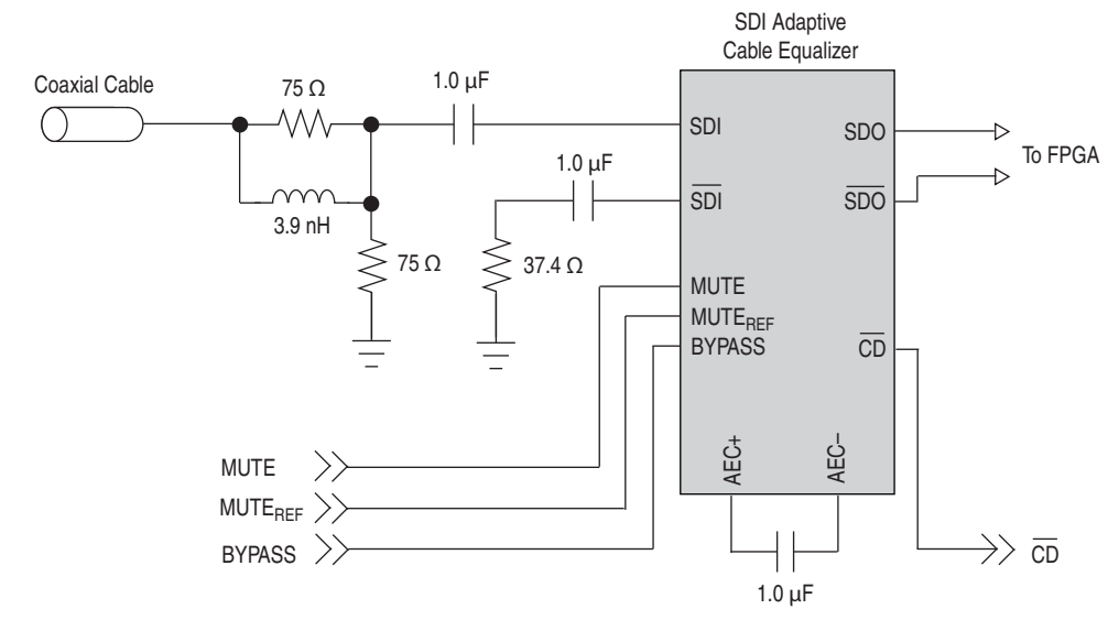
Figure 2-9. SDI Cable Equalizer
