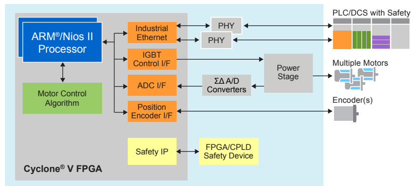
Figure 1: Cyclone V or Cyclone V SoC FPGAs: Single Drive Device Integrates High-Performance Processor Subsystem with Motor Control Algorithm, I/O Logic, Industrial Ethernet Protocols, and Safety Elements
