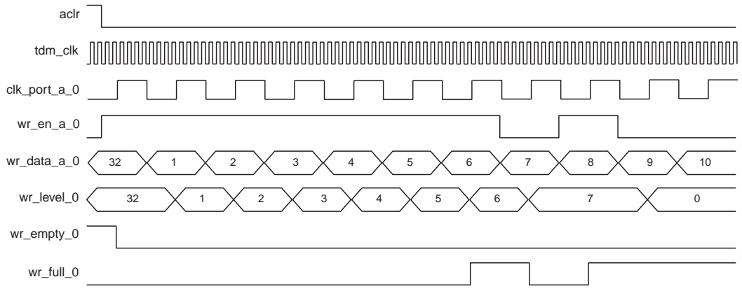
Figure 6. Initializing and Writing to a FIFO
