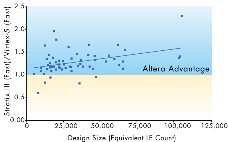
Figure 4. Stratix III FPGA Performance Advantage Increases With Design Size
