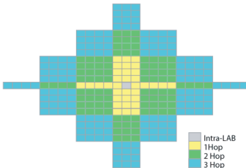
Figure 16. Stratix Series Connectivity
