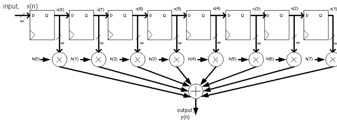
Figure 1: FIR Filter
