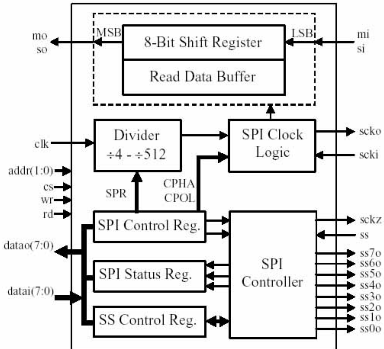
Figure 1. DSPI - Serial Peripheral Interface Master/Slave Block Diagram
