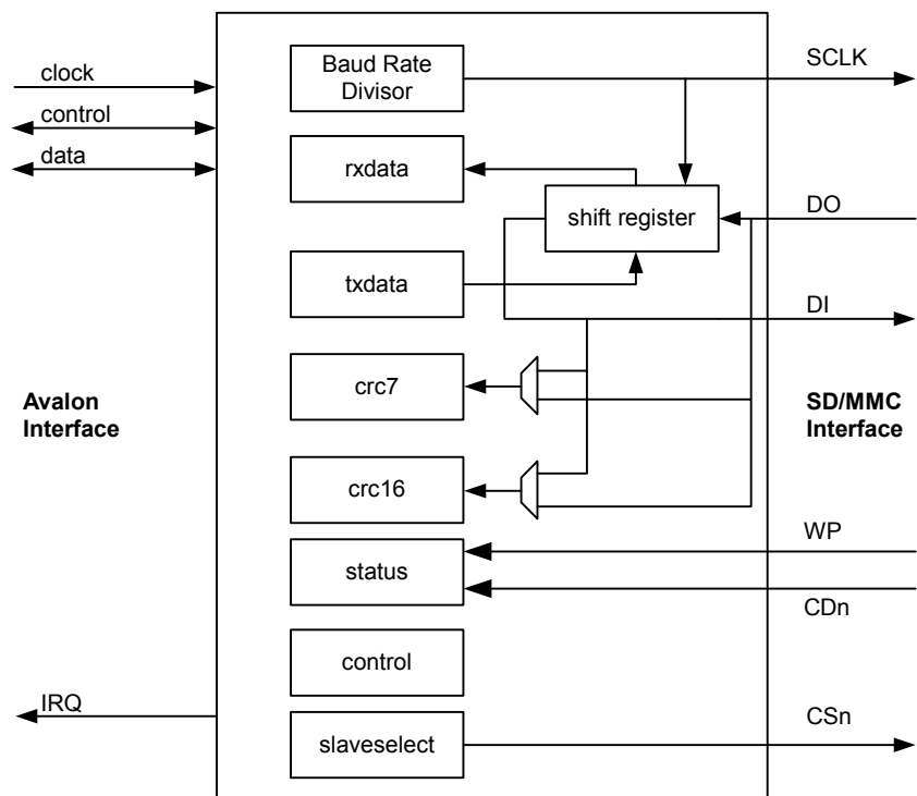
Figure 2: SD/MMC SPI Core Block Diagram
