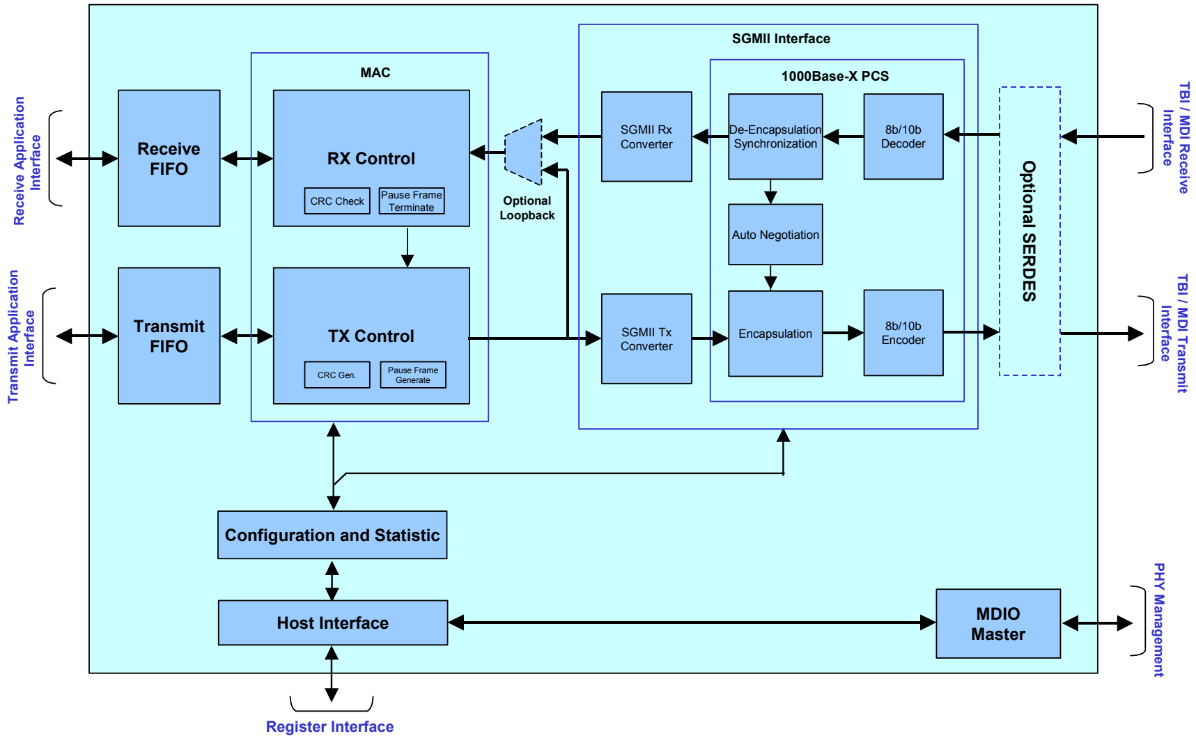
Figure 1. 10/100/1000 Ethernet MAC Core With SGMII
