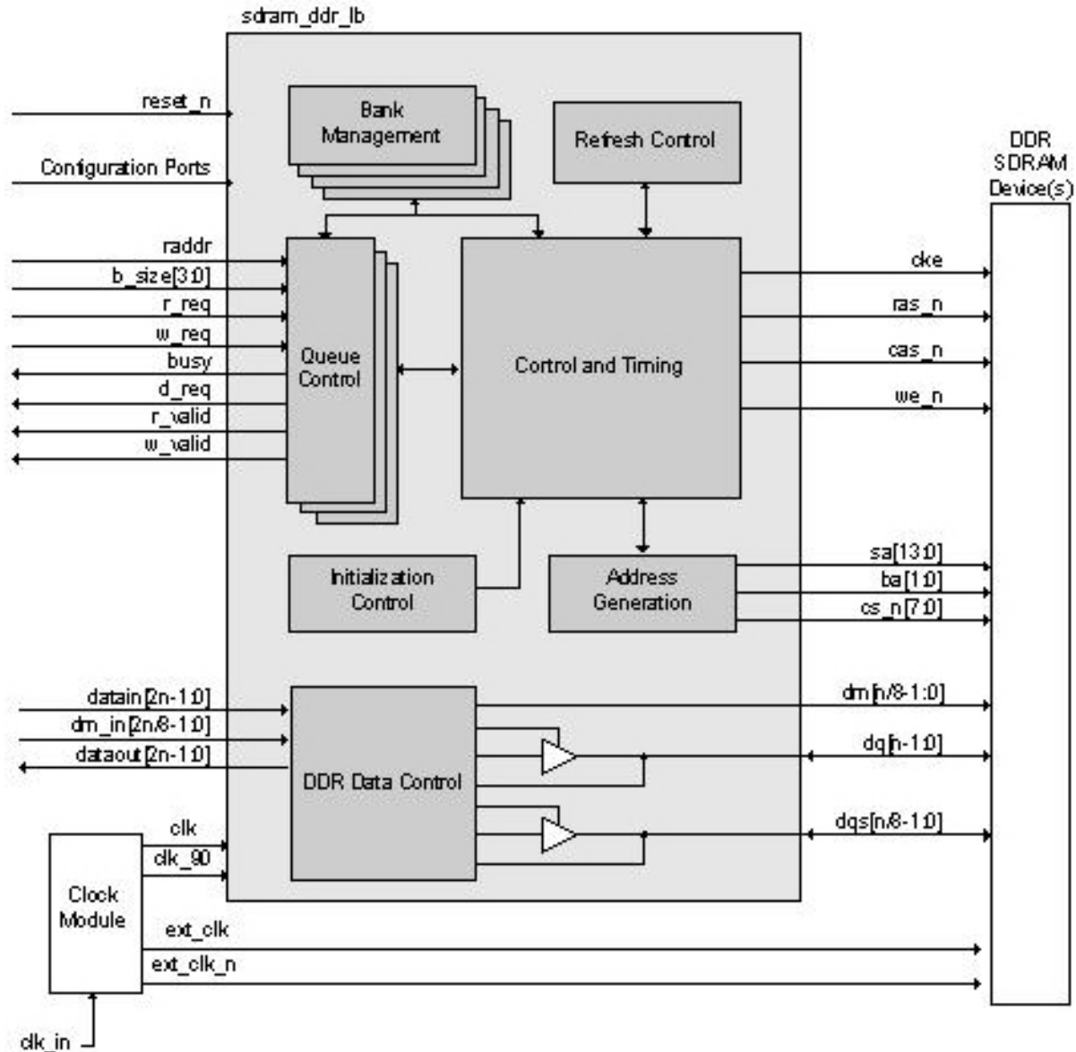
Figure 1. DDR SDRAM Controller Block Diagram
